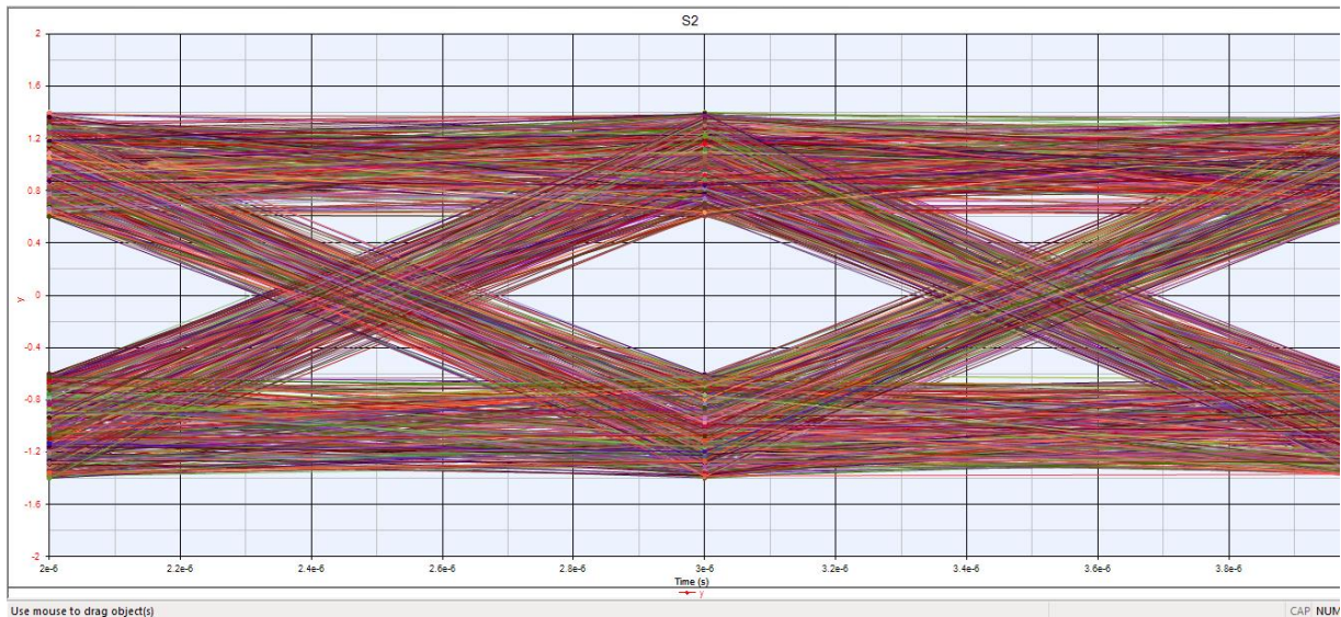
Figure 9.9. Eye diagram of the schematic in Figure 9.8.
