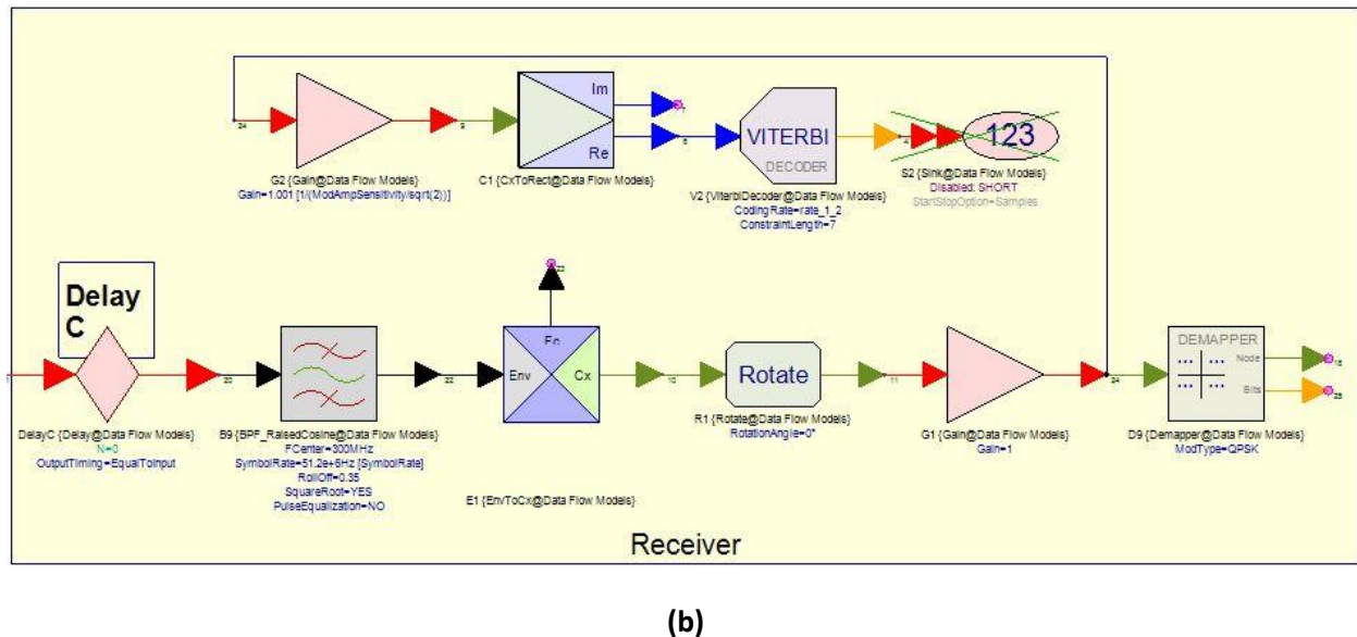
Figure 6.2. From schematic QPSK_Design. A shot of the transmitter (a) and a shot of the receiver (b).
