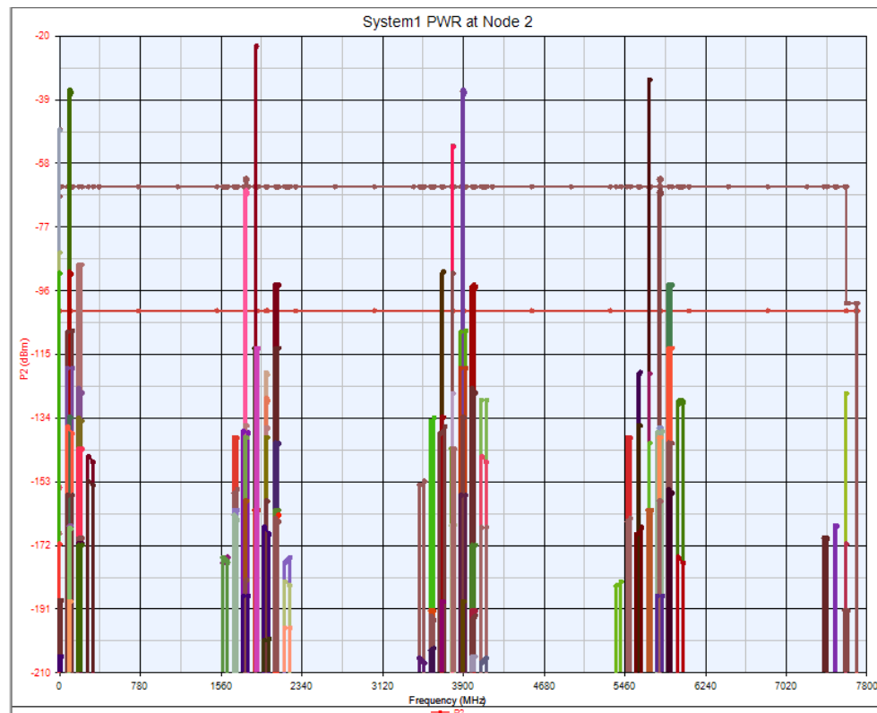
Figure 9.29. Power plot.
