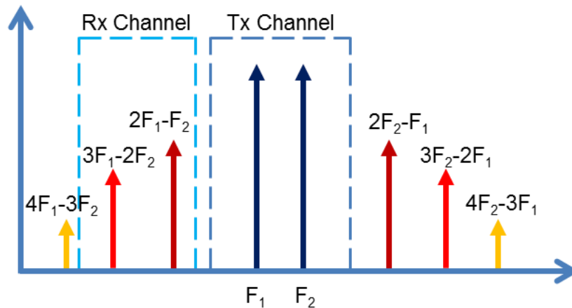
Figure 2.13. Intermodulation products.
