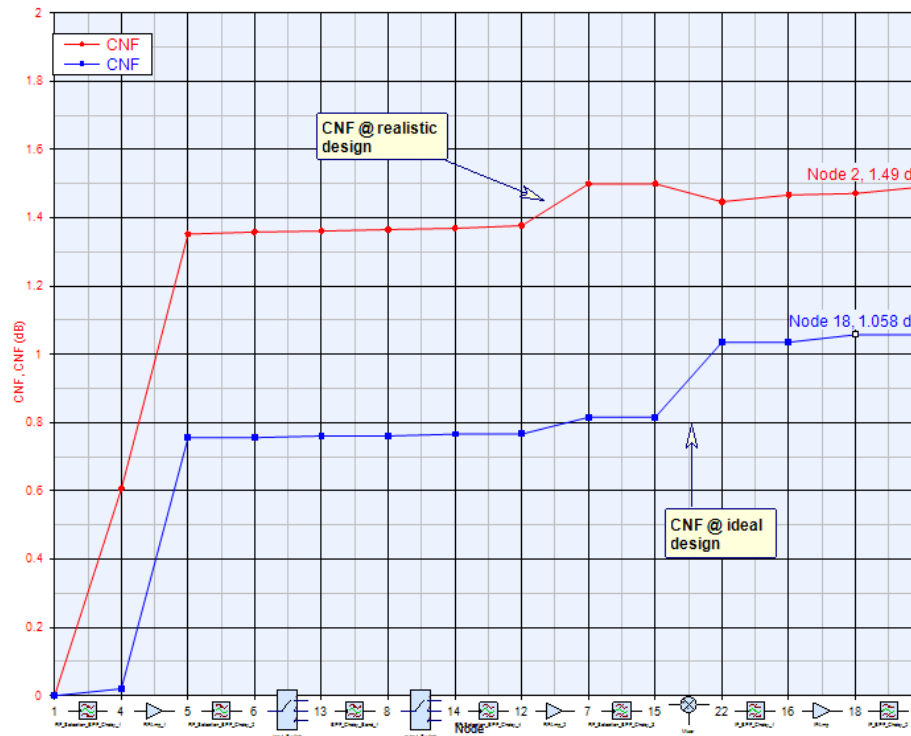
Figure 3.11. Cascaded Noise Figure (CNF) for band 1.
