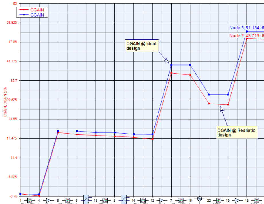
Figure 3.10. Cascaded Gain.
