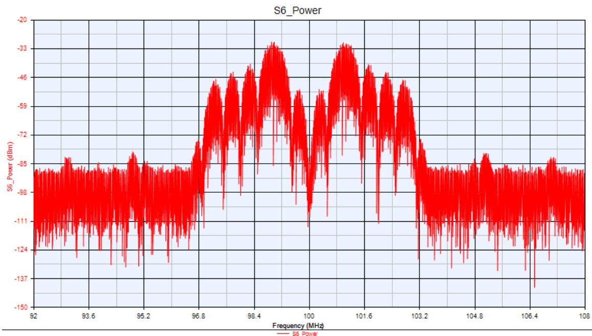
Figure 9.23. Power spectrum.
