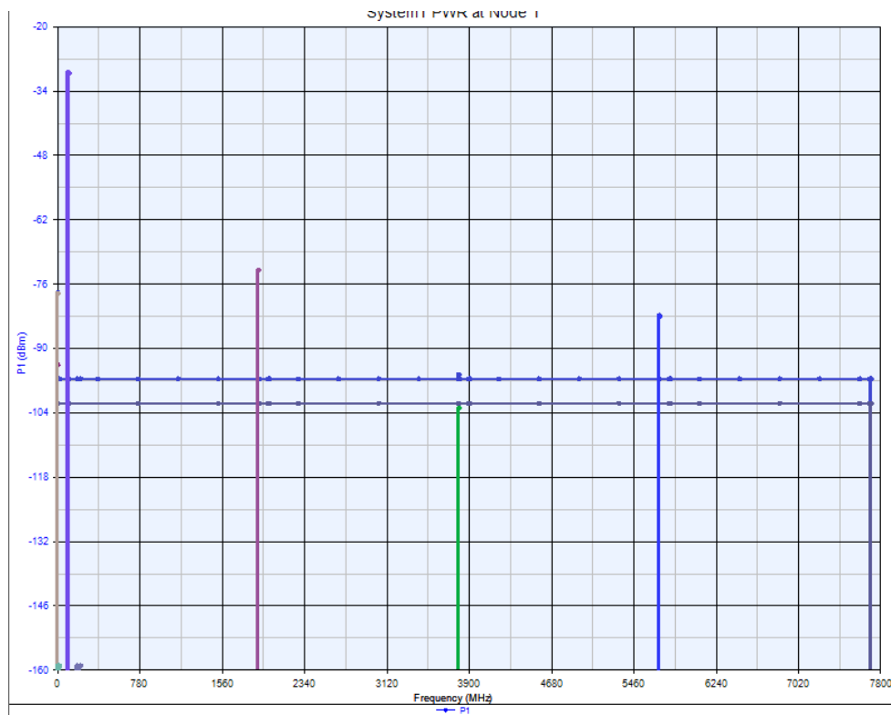
Figure 9.27. Power plot.
