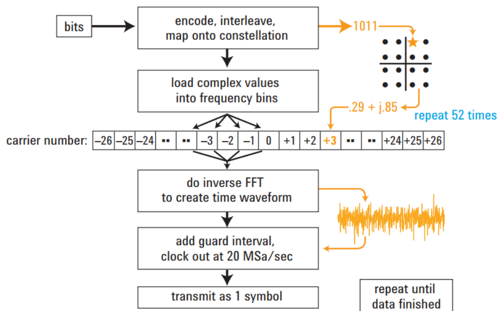
Figure 8.1. Example of an OFDM transmitting process.
