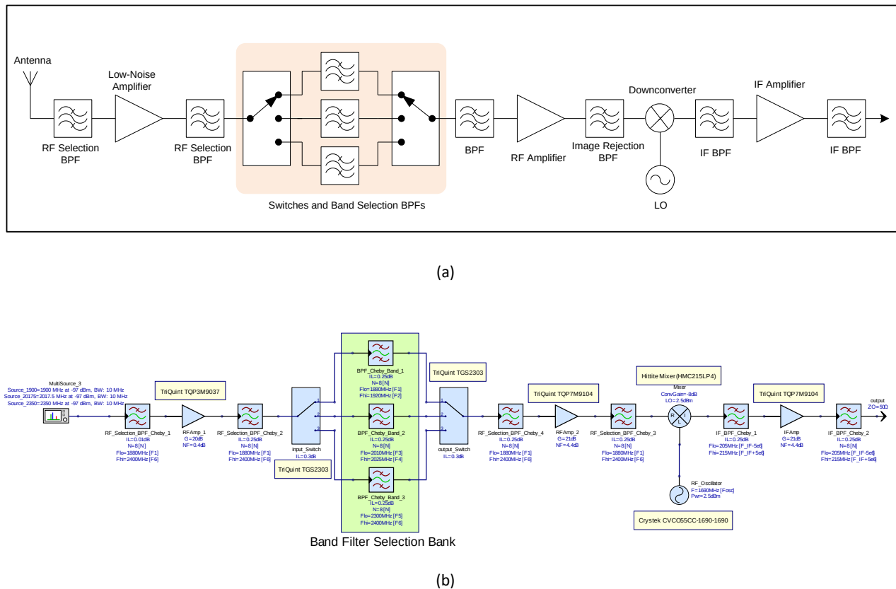
Figure 3.4. Proposed super-heterodyne architecture for the LTE receiver: (a) block diagram (b) PathWave System Design (SystemVue) model.
